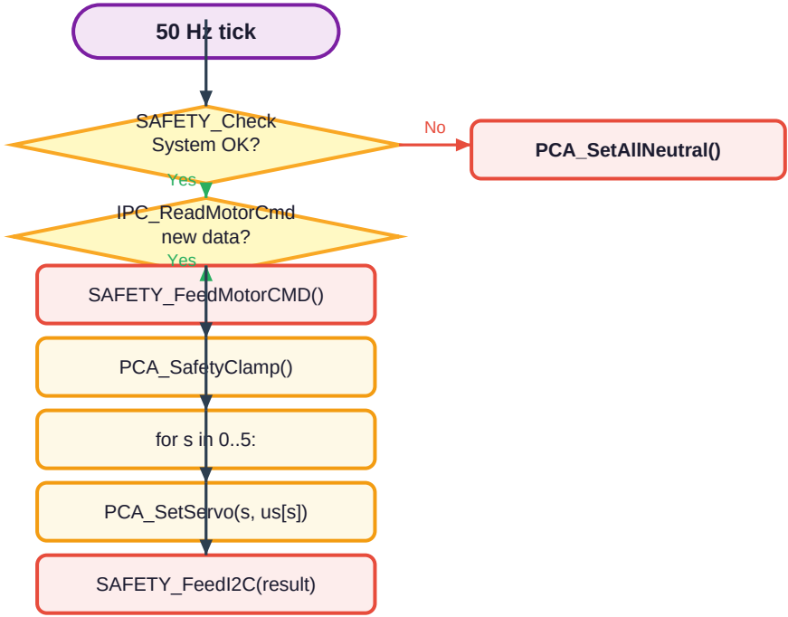
Servo Update Flowchart (50 Hz, in cpcu_io)
