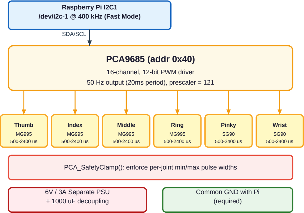
PCA9685 I2C Servo Driver Block Diagram
