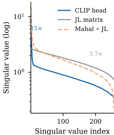
(a) Spectral gap
