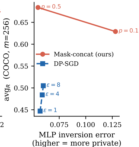
(c) Privacy-utility frontier
