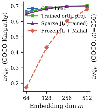
(b) Dimension scaling
