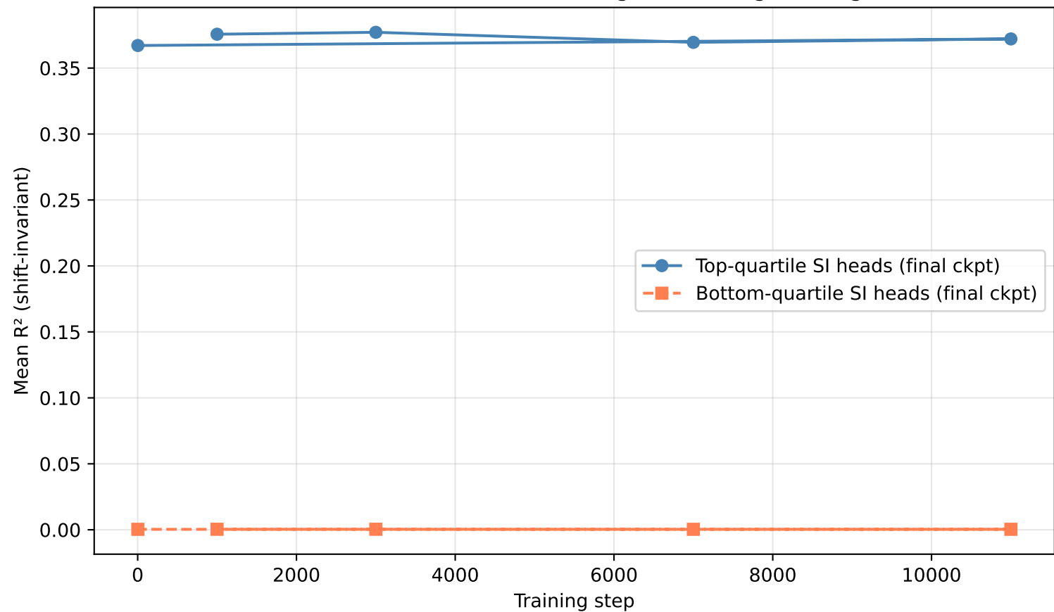
OLMo-2-7B SI Structure Emergence During Training
