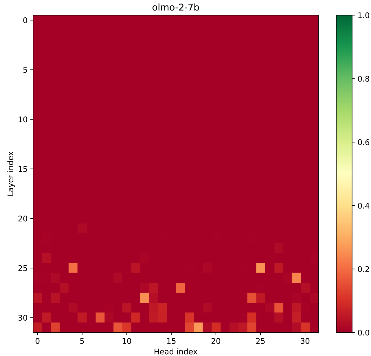
Boundary Attention Score by Layer and Head
