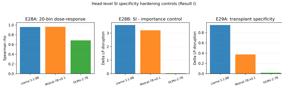
Figure 3: Head-level dose-response and specificity controls (primary finding). Left: 20-bin Spearman correlation between per-head R^2 and disruption cost under SI-kernel subtraction (Llama \rho=0.959 , Mistral \rho=0.964 , OLMo \rho=0.684 ; all one-tailed permutation p < 0.001 ). Center: SI-ranked intervention minus importance-matched non-SI intervention (positive in all three models, ruling out generic head-importance as the driver). Right: Kernel-transplant specificity — transplanting norm-matched high-SI kernels onto low-SI heads versus low-head self-subtraction (positive in all three models).
