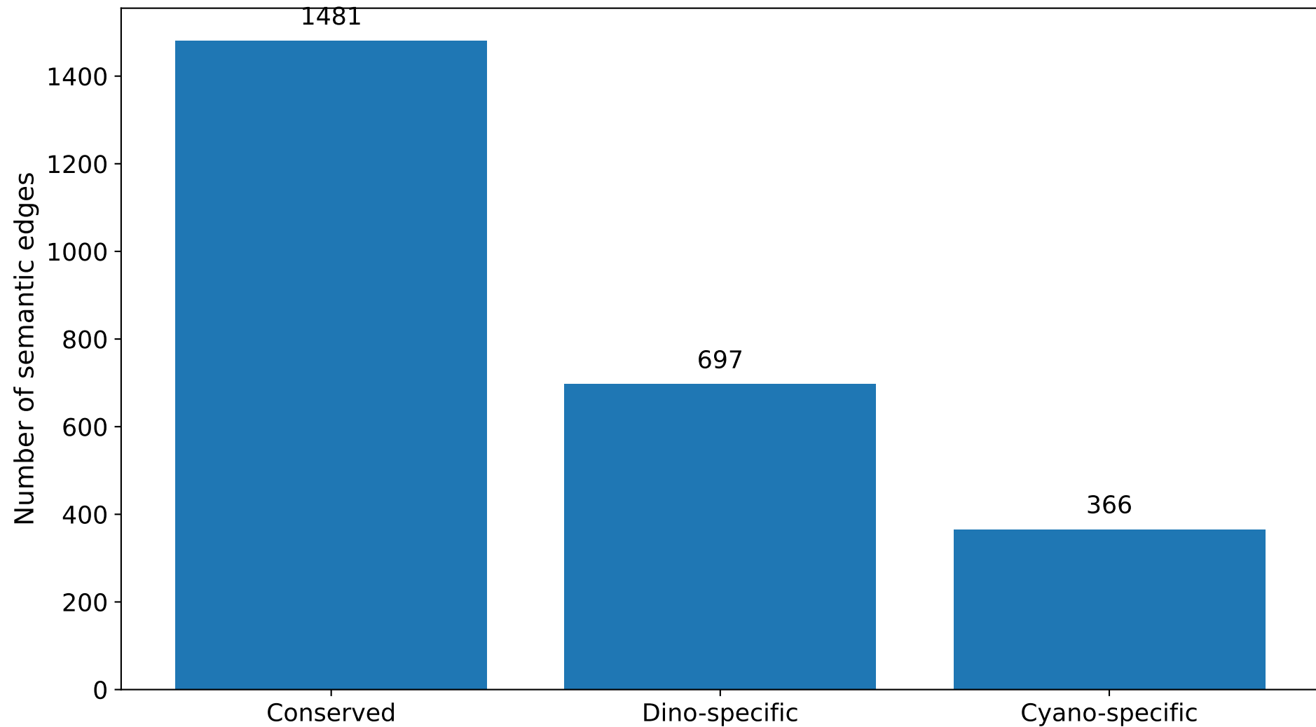
Conserved vs divergent cross-taxa STX semantic edges
