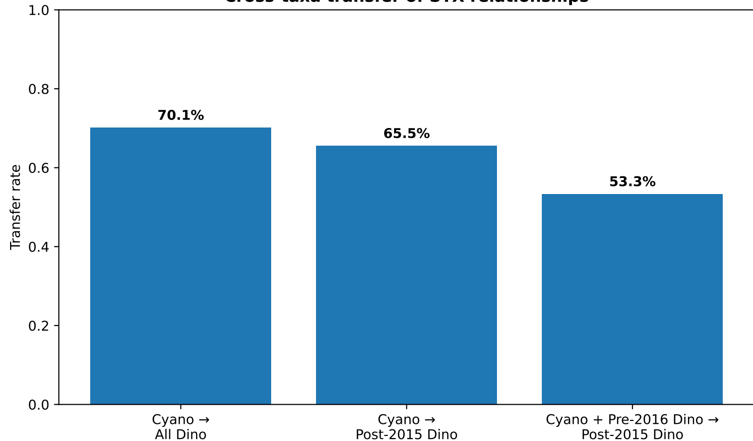
Cross-taxa transfer of STX relationships
