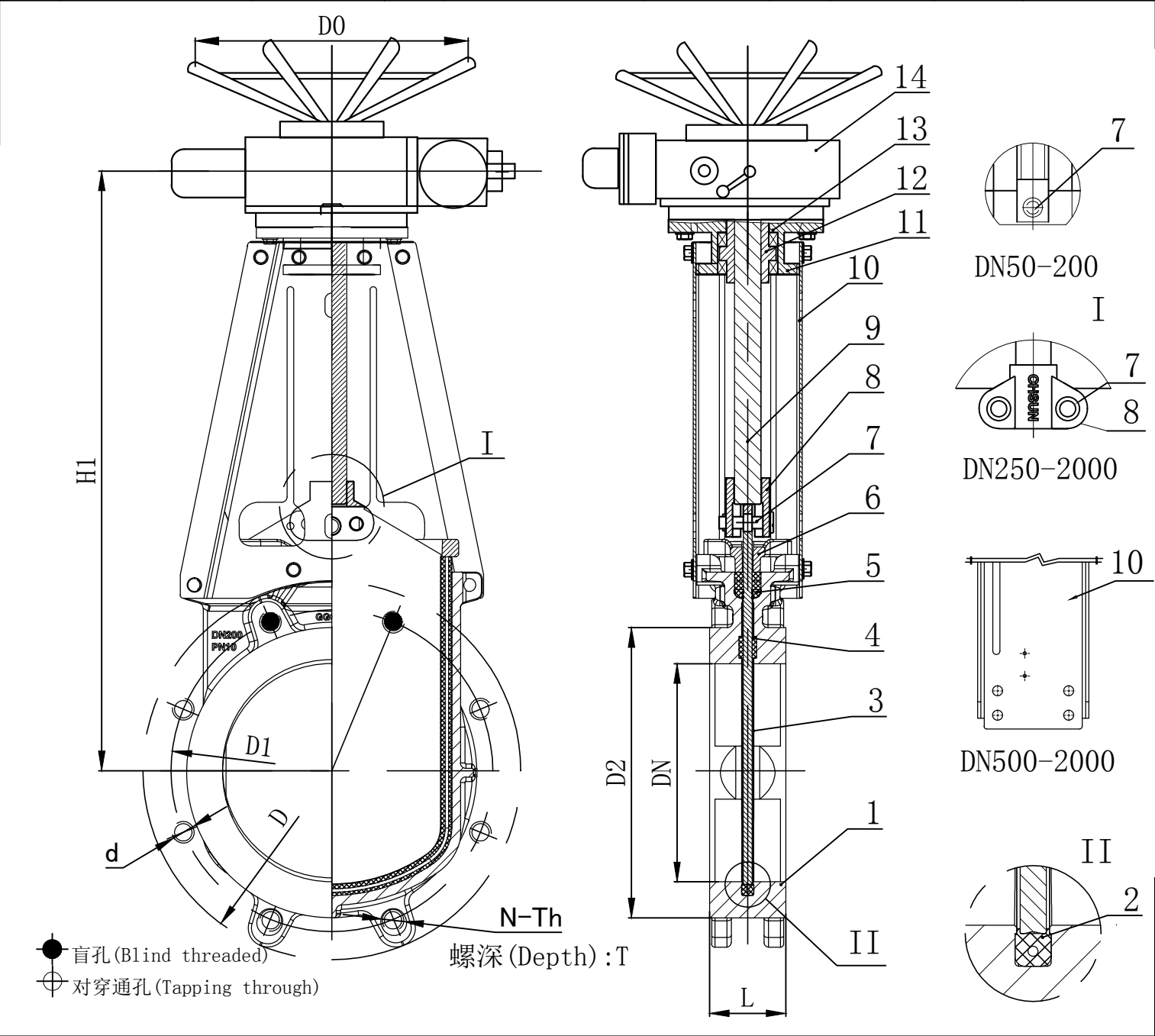
刀闸阀 Knife Gate Valve
