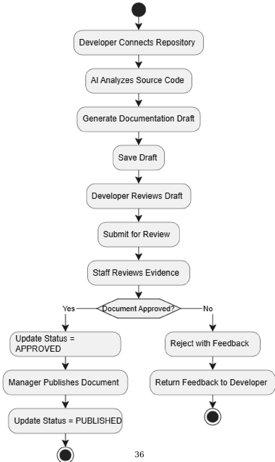
Figure IV.1: AI Documentation Generation Activity Diagram
