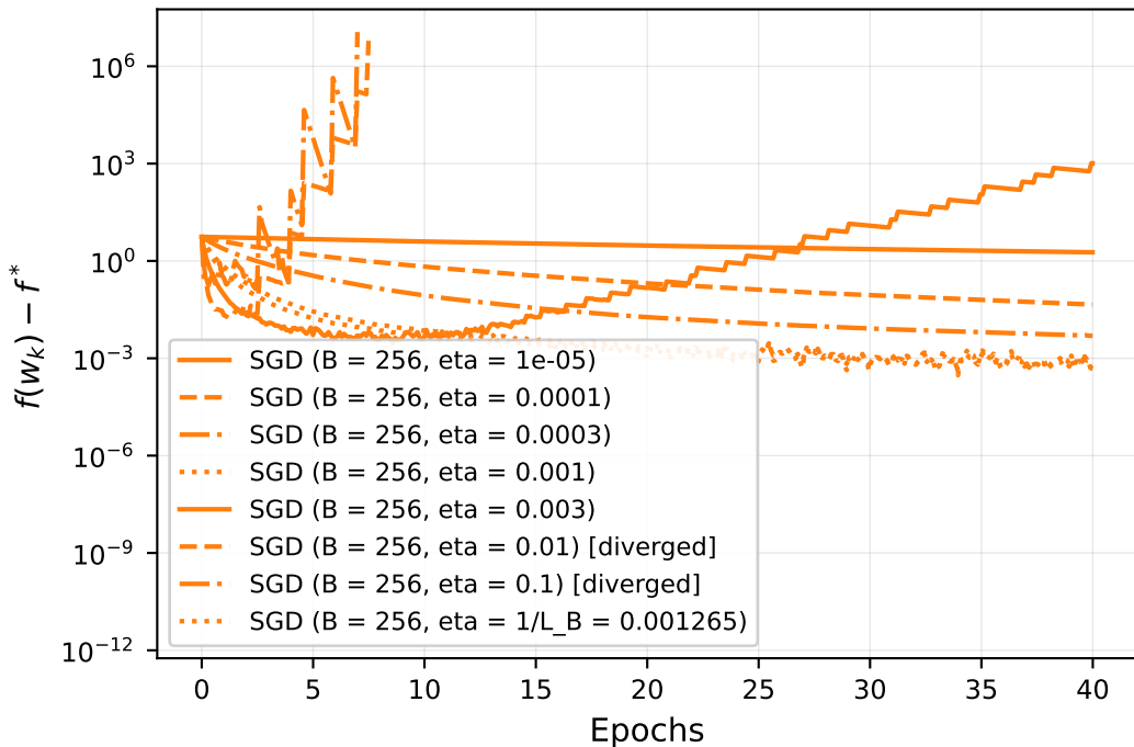
Initial step sizes for SGD
