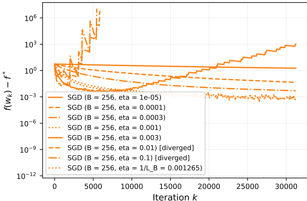
Initial step sizes for SGD
