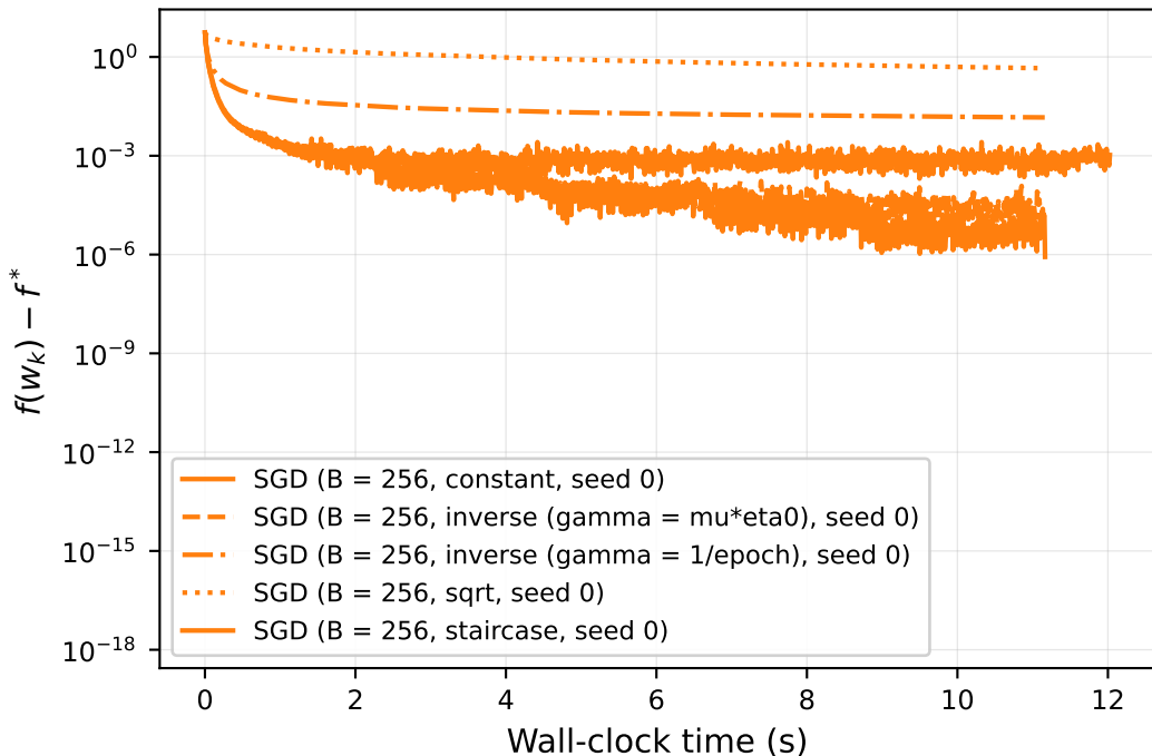
Step-size schedules for SGD
