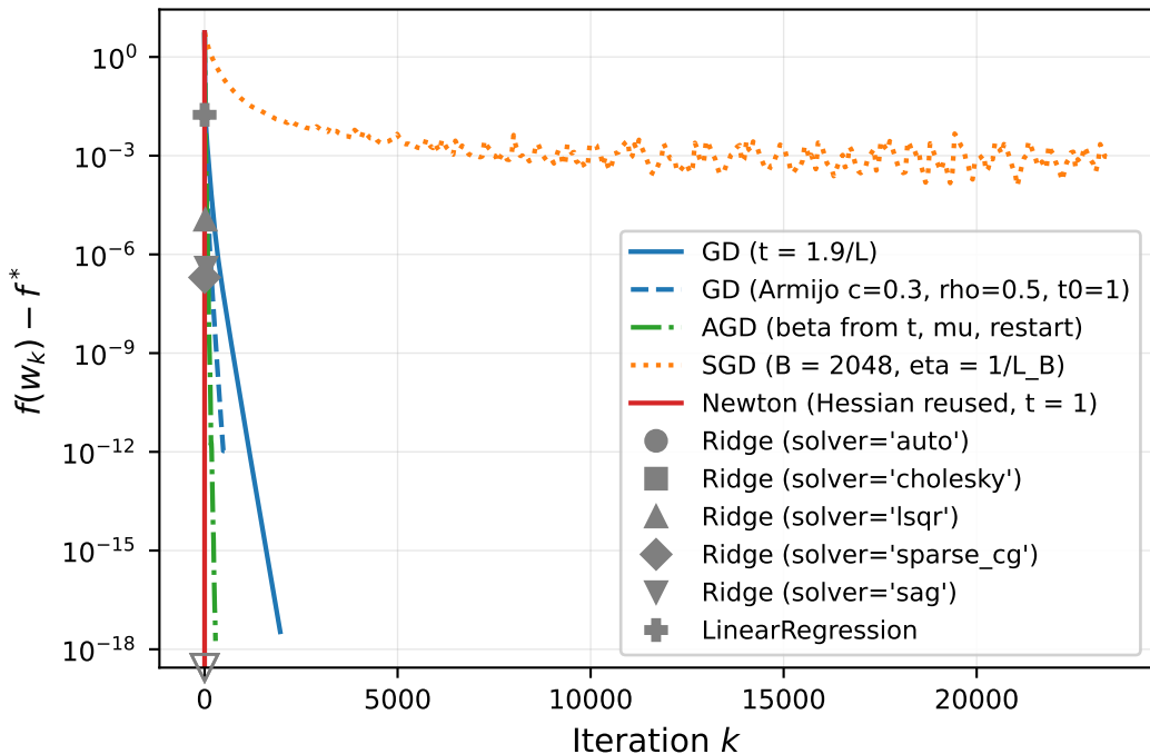
Ours vs scikit-learn, n = 1,200,000
