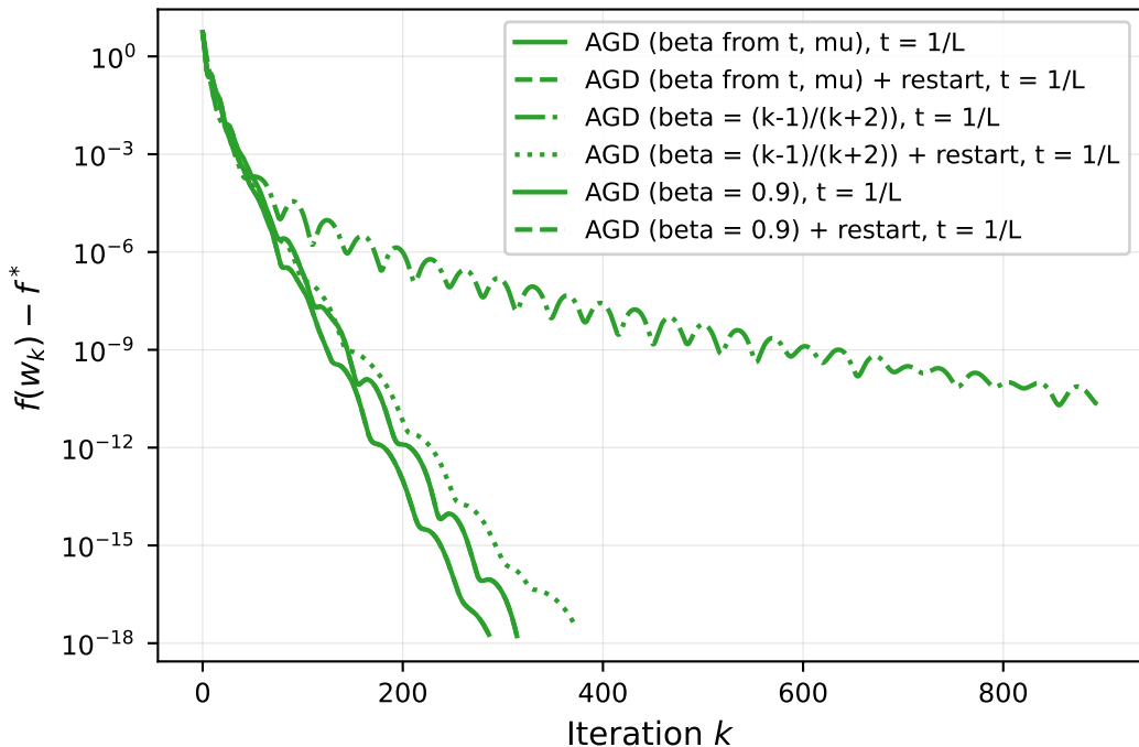
Adaptive restart on and off
