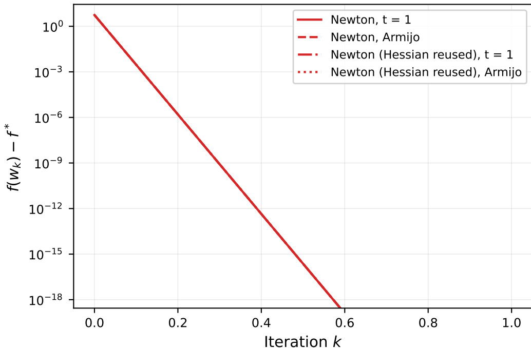
Newton: cost of rebuilding the Hessian, n = 1,200,000
