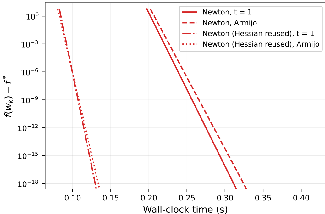
Newton: cost of rebuilding the Hessian, n = 1,200,000
