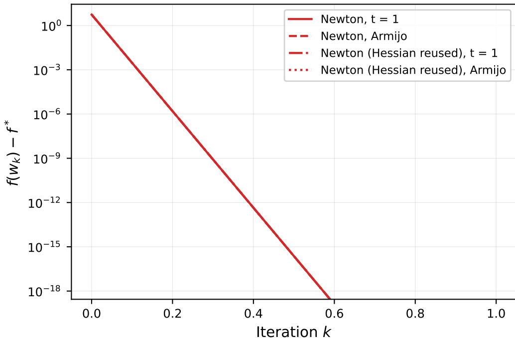
Newton: damping and Hessian reuse
