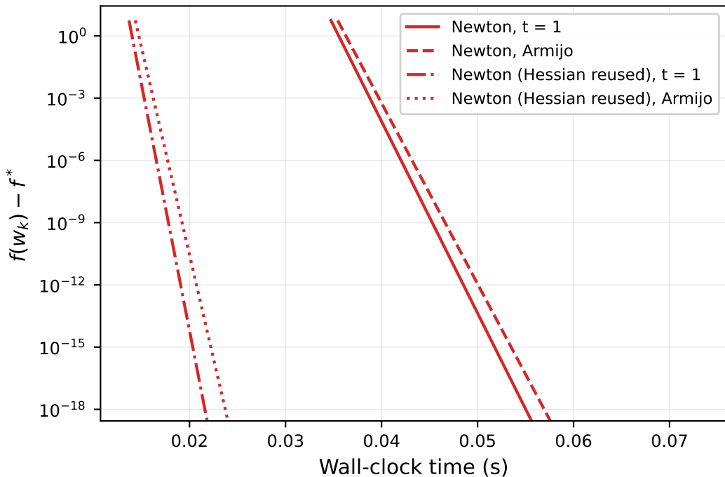
Newton: damping and Hessian reuse
