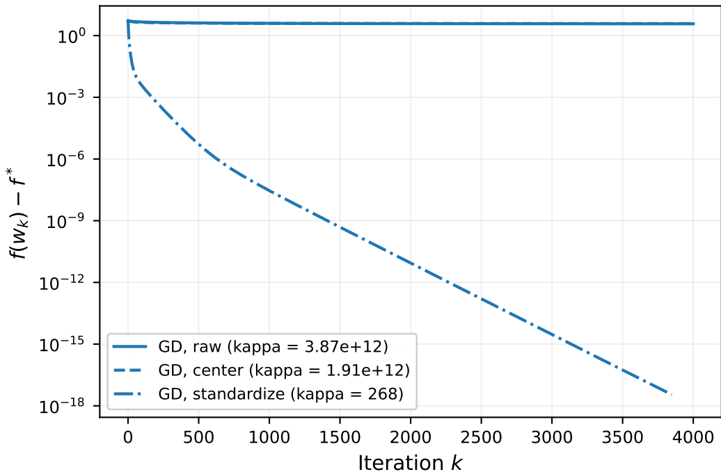
Column scaling and the conditioning
