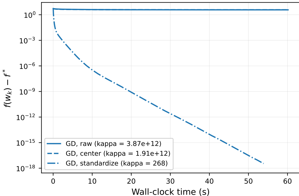
Column scaling and the conditioning
