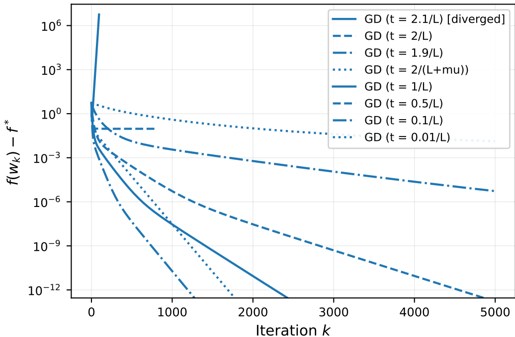
Constant step sizes for gradient descent
