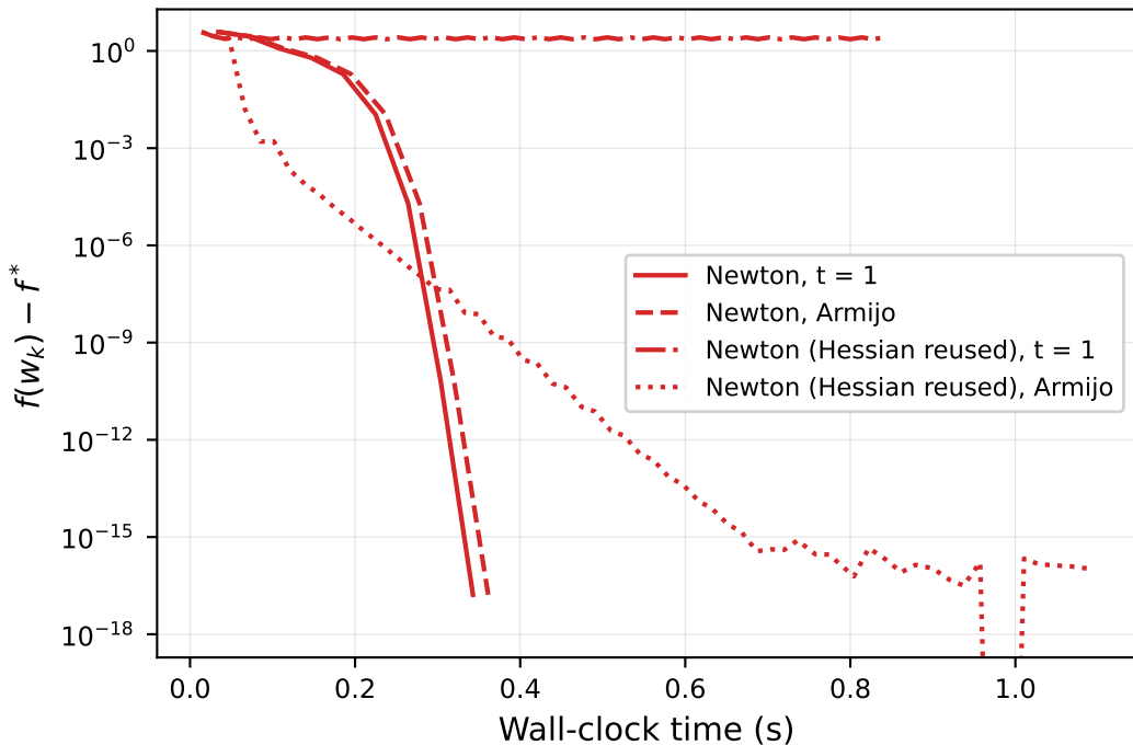
Newton on the Huber objective
