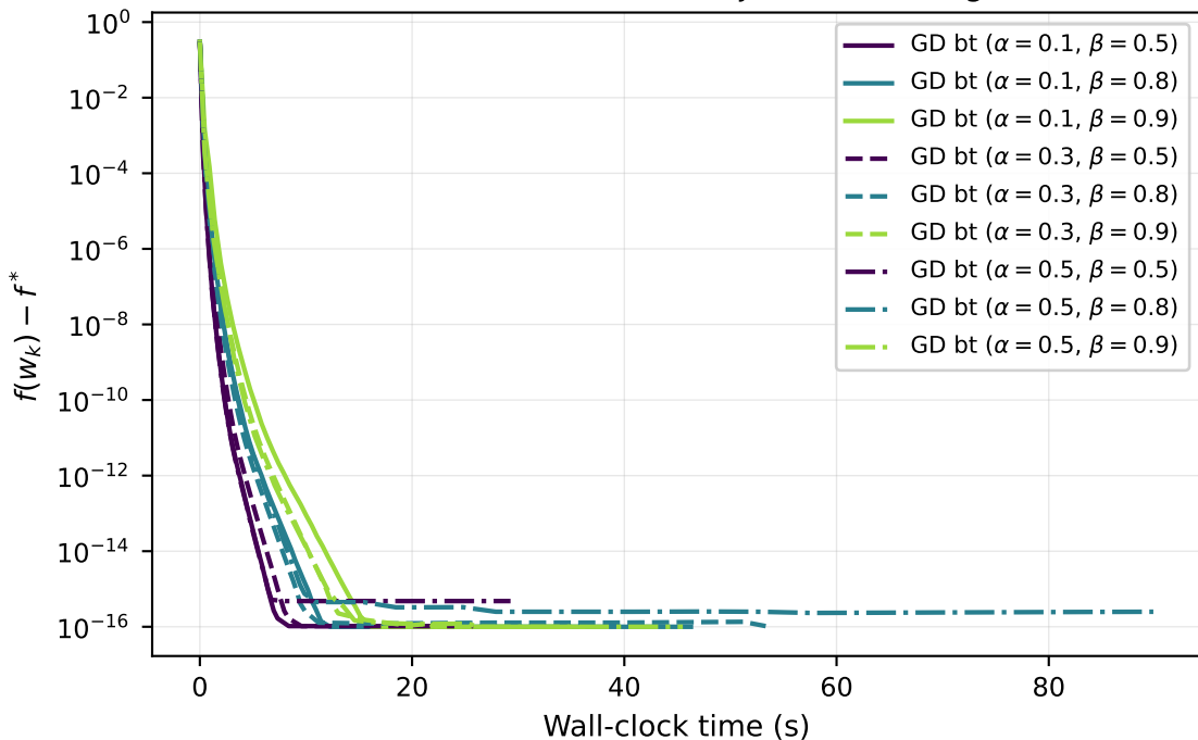
Gradient descent: Armijo backtracking
