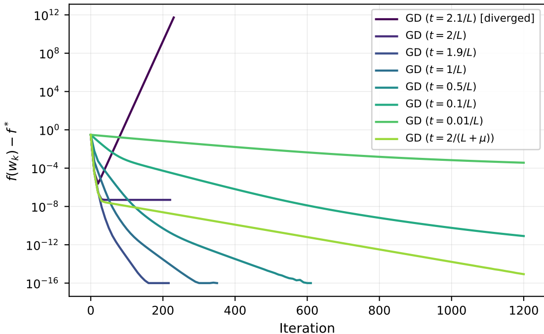
Gradient descent: fixed step sizes
