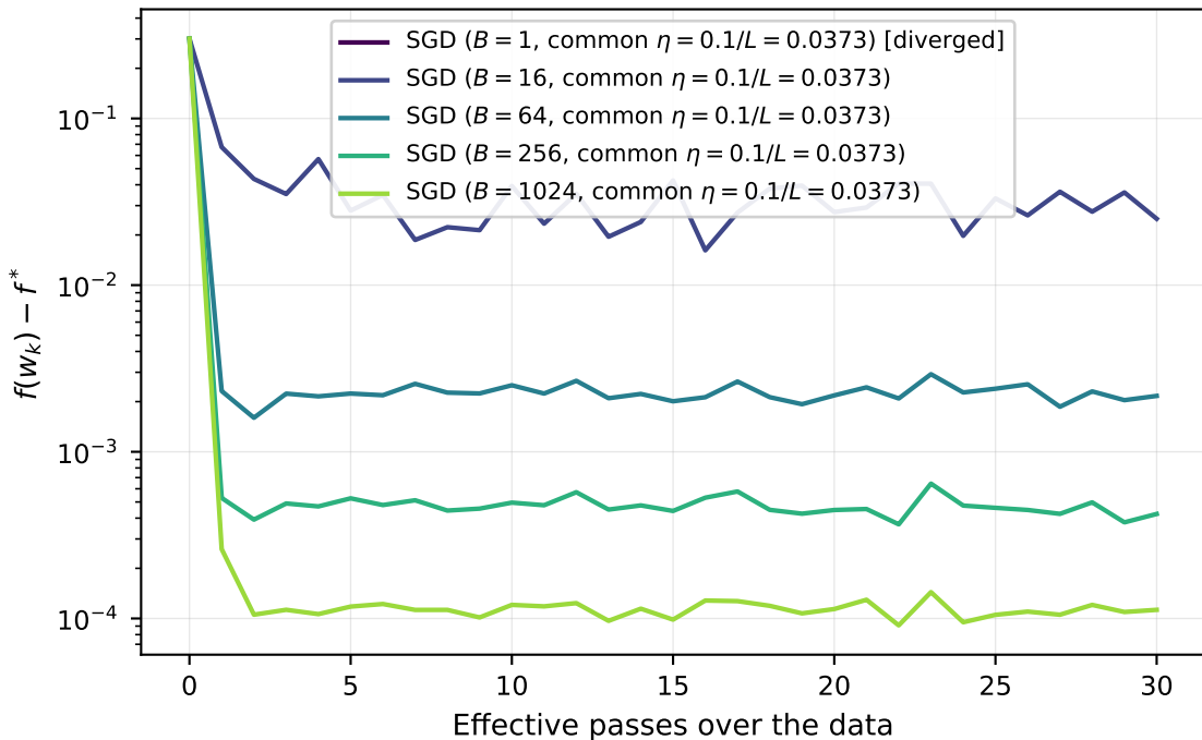
SGD: one common step size for every batch size
