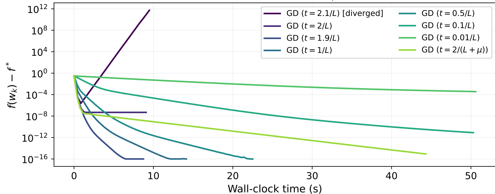
Gradient descent: fixed step sizes
