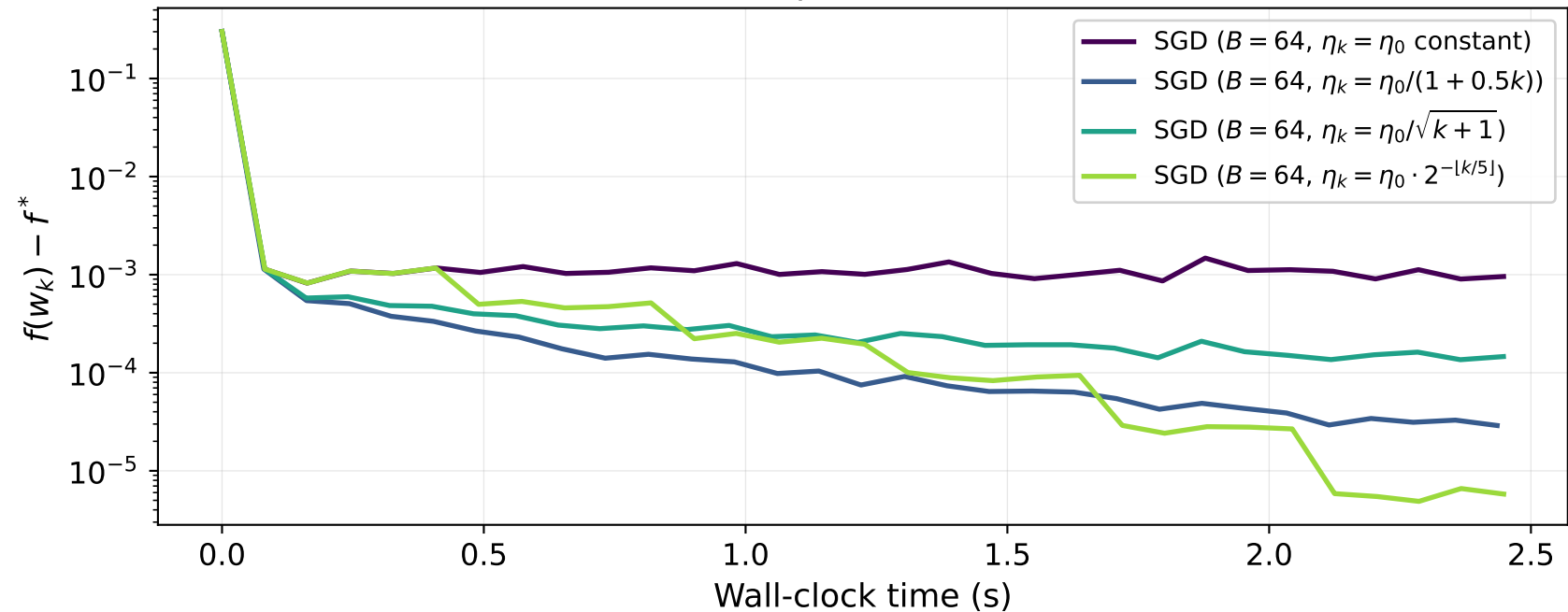
SGD: step size schedules
