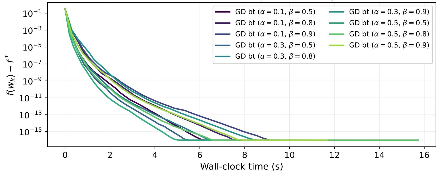
Gradient descent: Armijo backtracking
