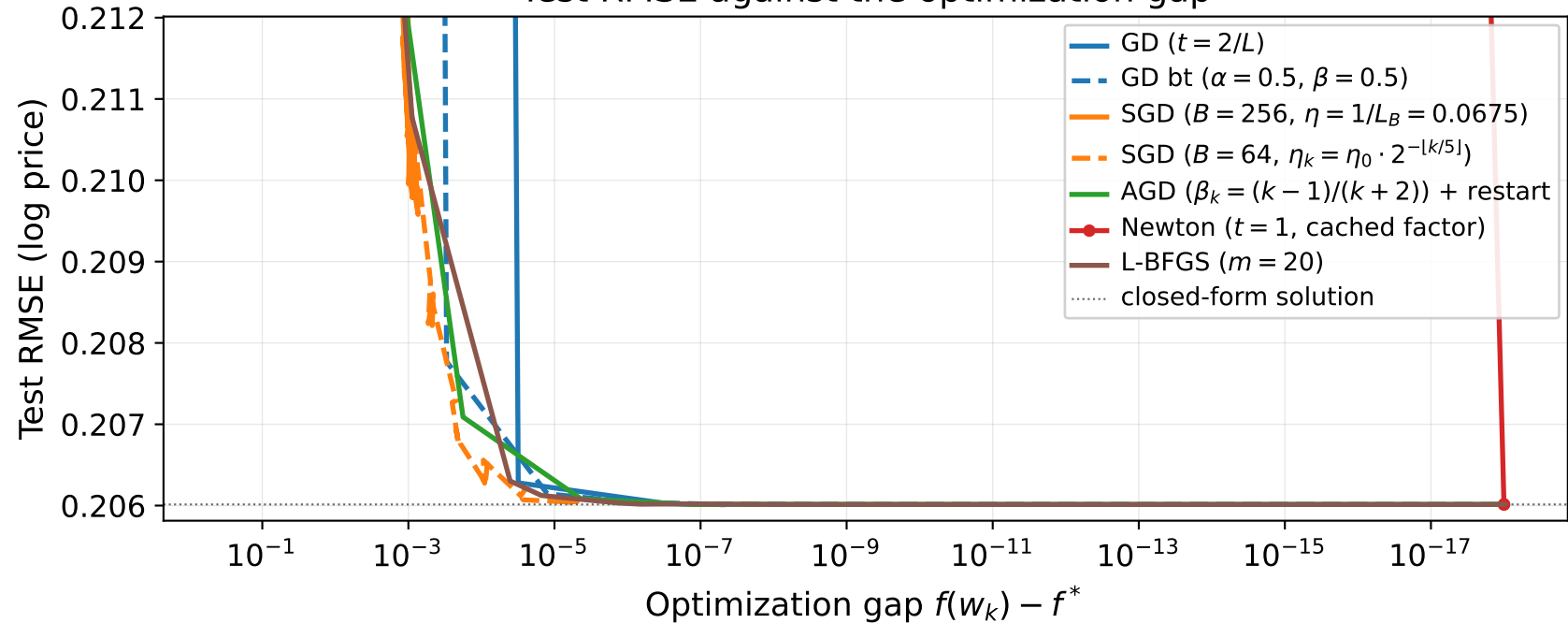
Test RMSE against the optimization gap
