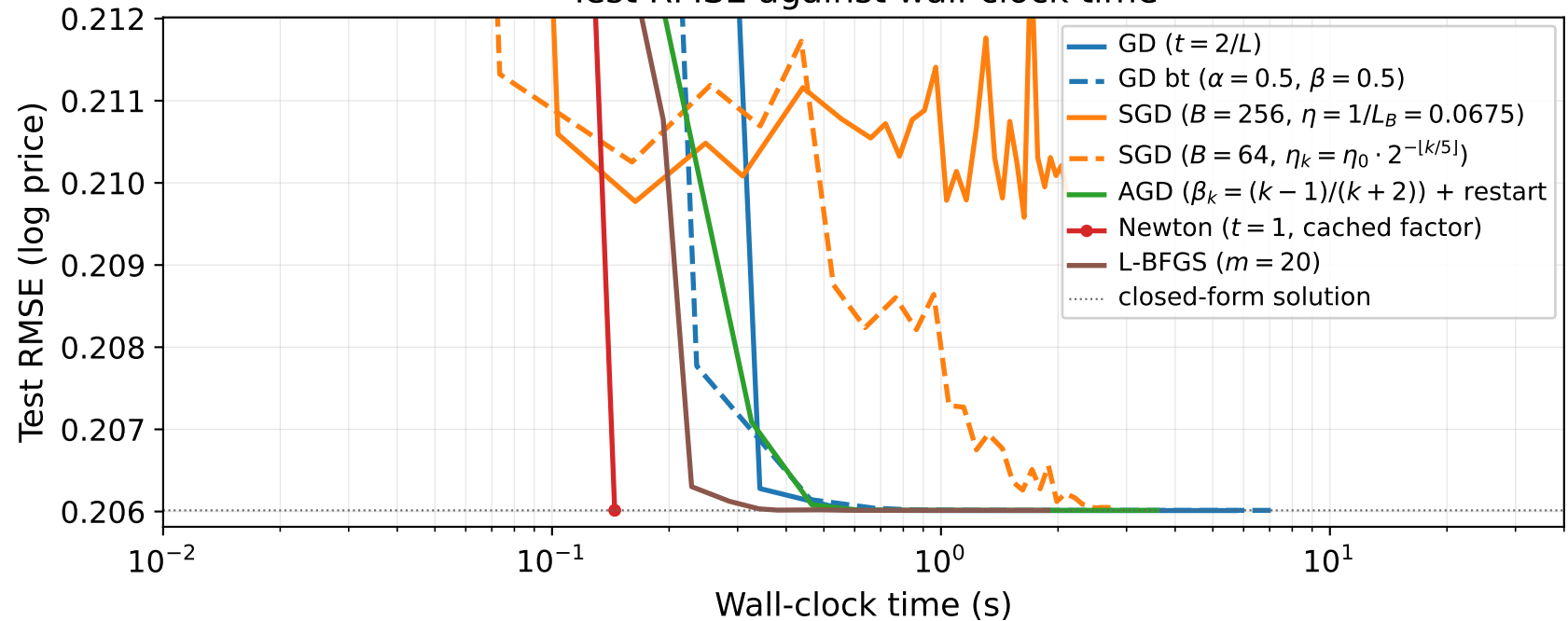
Test RMSE against wall-clock time
