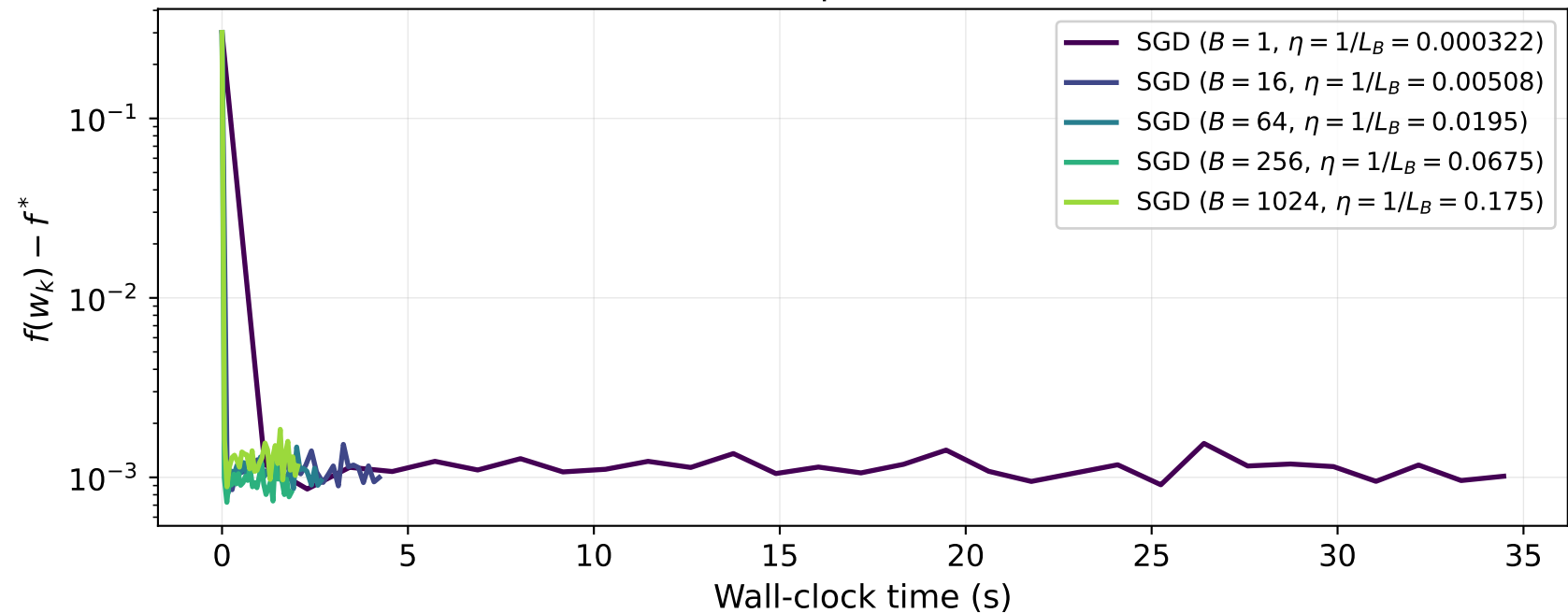
SGD: batch size, step matched to each batch
