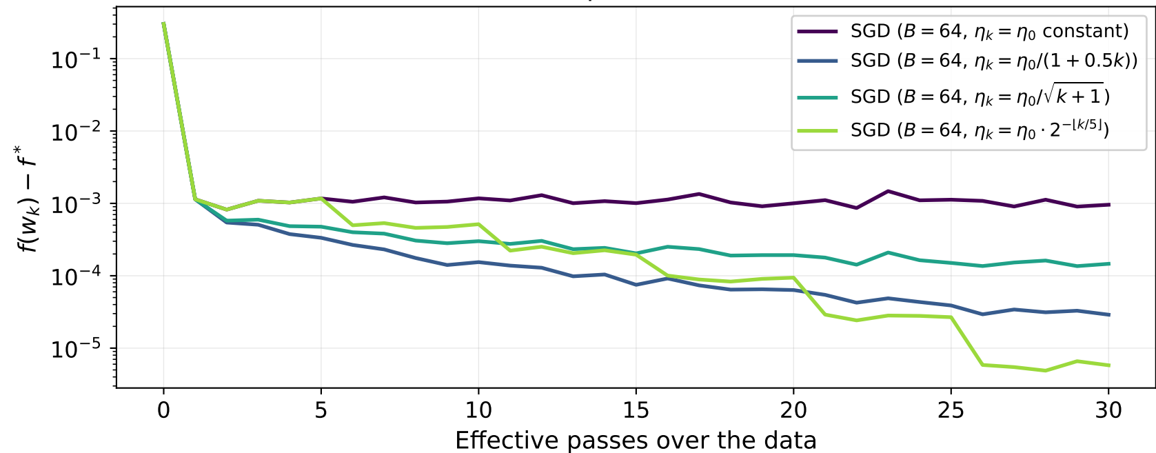
SGD: step size schedules
