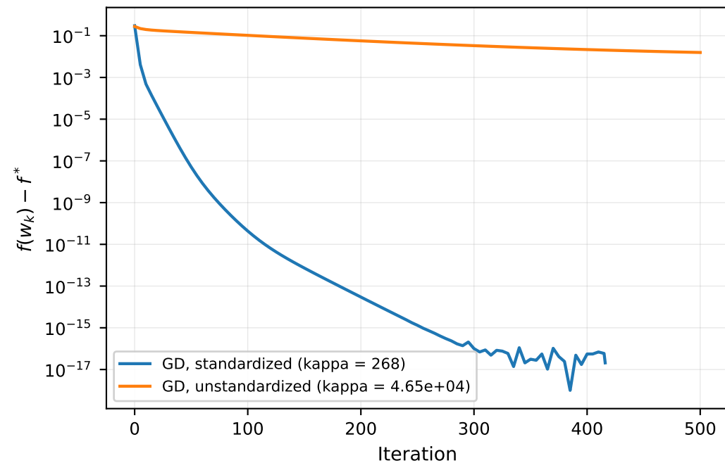
Effect of column standardization on the convergence rate
