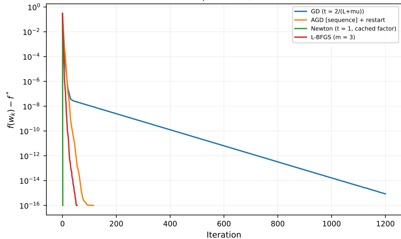
Hand-written optimizers (iteration axis)
