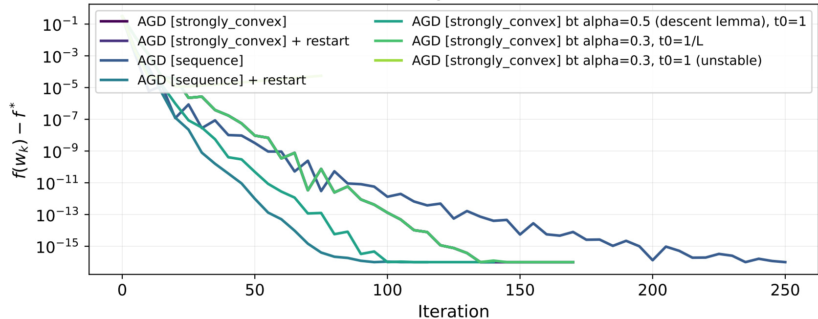
Accelerated gradient descent
