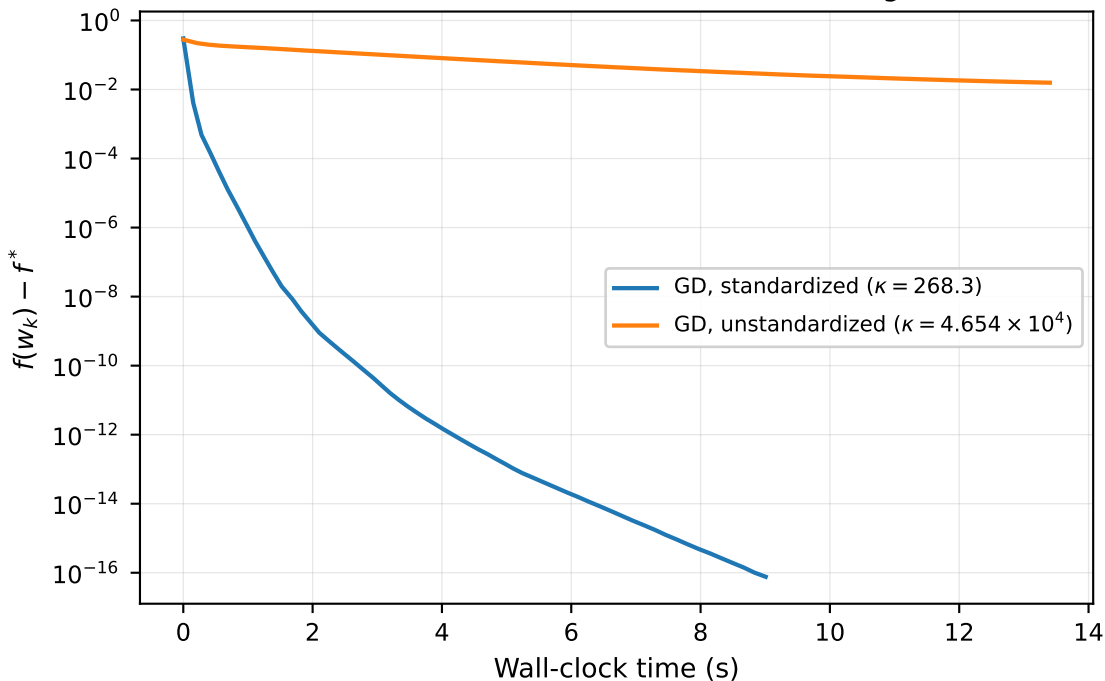
Effect of column standardization on the convergence rate
