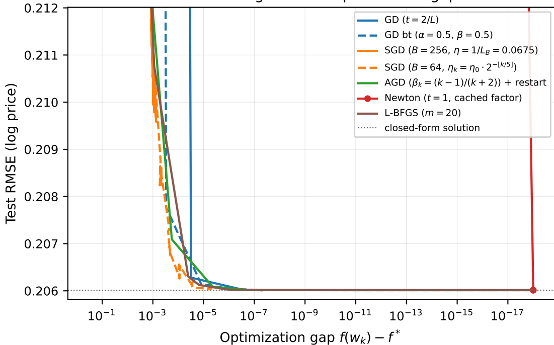
Test RMSE against the optimization gap
