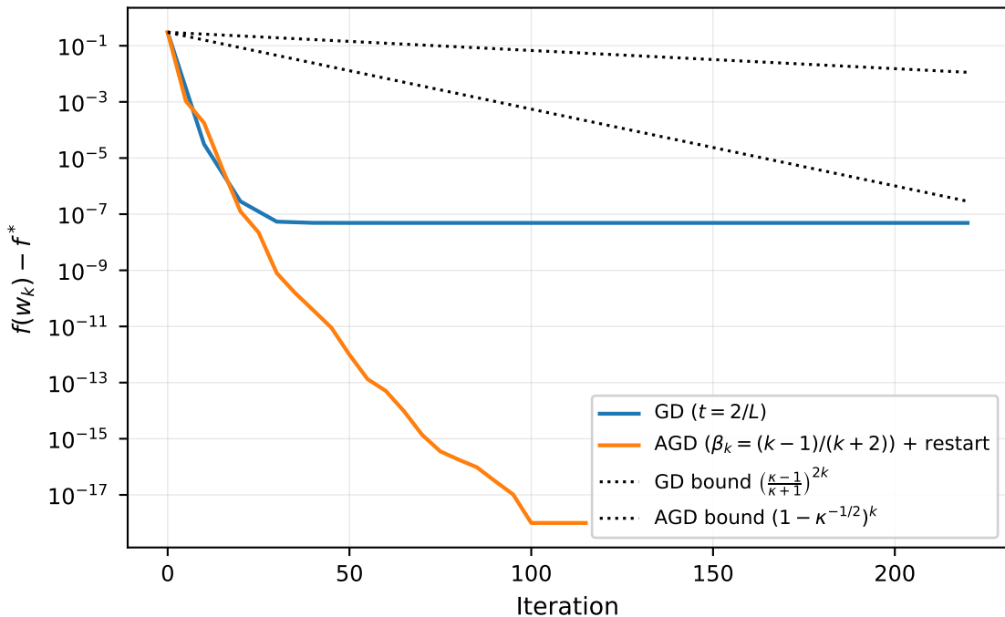
Observed convergence against the theoretical bounds
