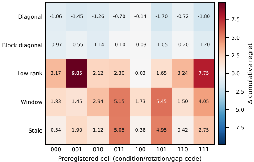
(b) Paired method-minus-full regret
