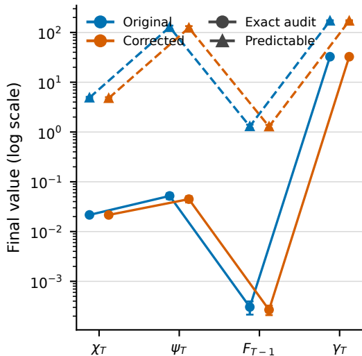
(a) Exact vs. predictable certificates
