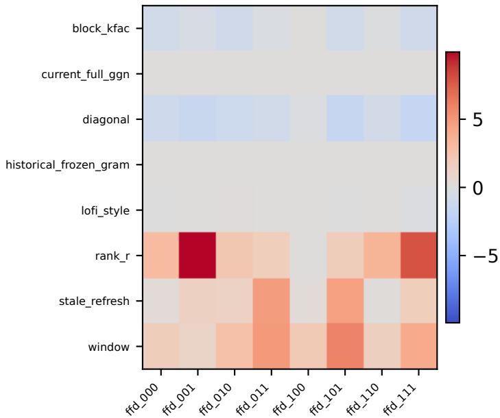
identical theoretical
