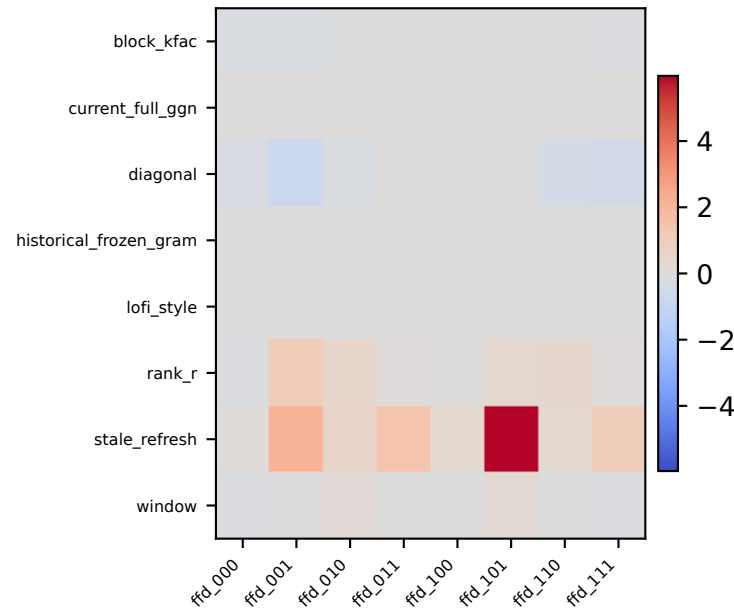
matched 95 coverage
