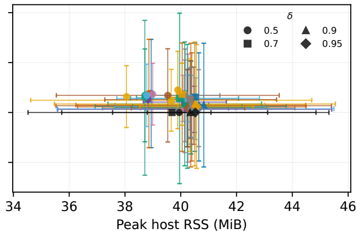
Memory versus regret
