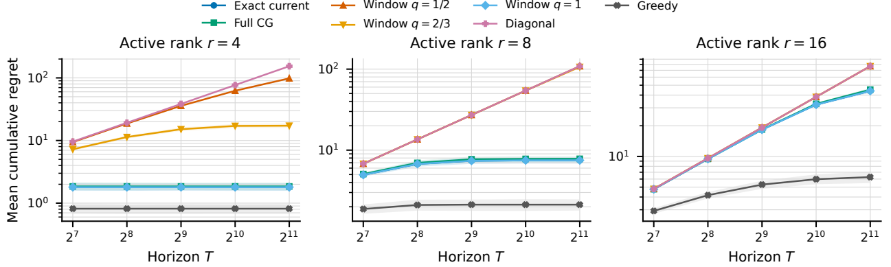
Figure 1: Finite-horizon theorem-scaling diagnostic at ambient dimension d = 2048 . Curves are 50-seed mean cumulative regret with paired-seed bootstrap 95% intervals at the five preregistered trajectory prefixes. Full CG uses the residual-checked ambient CVP implementation; greedy is an uncertified control. The fitted log-log behavior is descriptive and does not prove an asymptotic rate.
