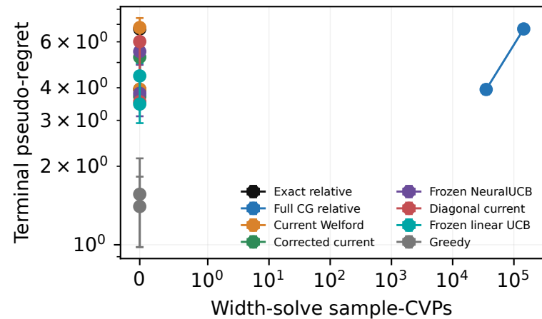
Regret versus solve work
