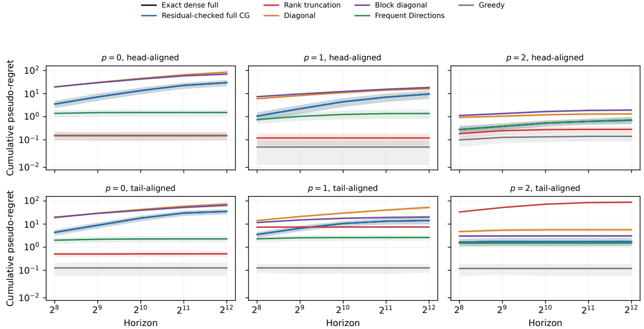
Figure 1: Full spectral-tail evaluation at d = 256 , K = 8 , and displayed rank r = 8 . Curves are means over untouched evaluation seeds 1000–1049; bands are 95% whole-seed bootstrap intervals at five predeclared horizons. Bonuses are selected on tuning seeds 0–9 over the complete predeclared cell set. Head- and tail-aligned regimes include cells unfavorable to full curvature.
