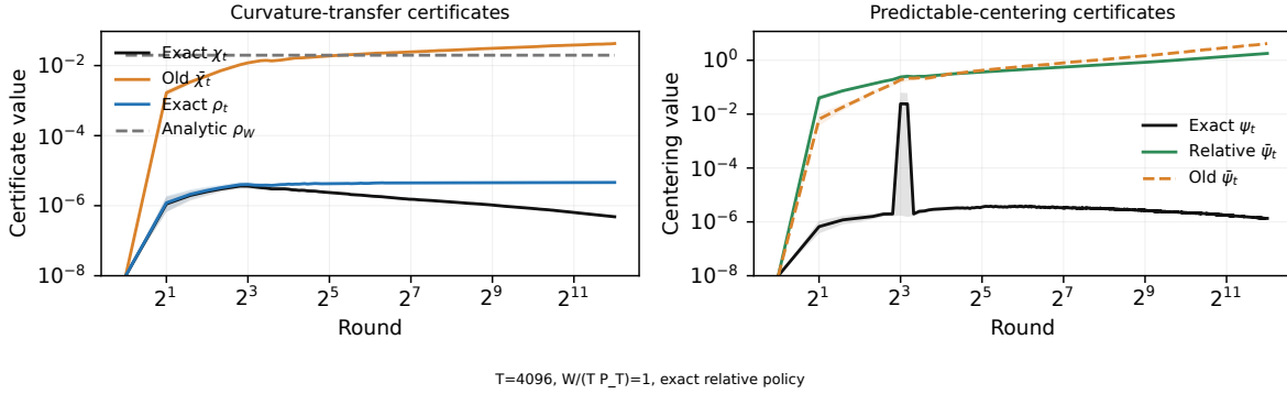
Figure 3: Final-holdout scaled-tanh certificate audit over five horizons, four width ratios, and 50 seeds. The displayed certificates are computed from complete trajectories, but every theorem-labeled method-cell fails the recorded joint theorem-event criterion. Transfer flags within the declared float64 tolerance are separated from analytic premise failures. This is a failure audit, not an empirical instantiation of Corollary 18.
