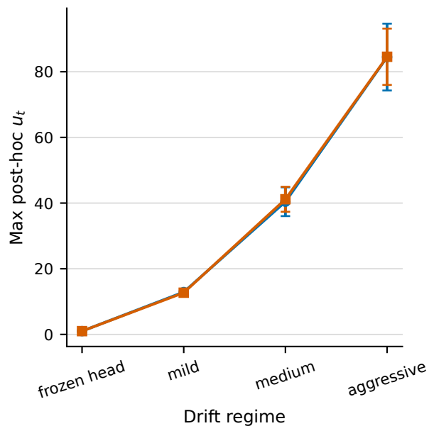
(e) Feature-drift transfer audit
