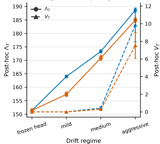
(f) Dynamic-complexity audit
