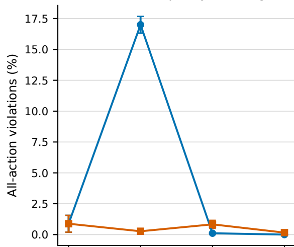
(e) Feature-drift transfer audit
