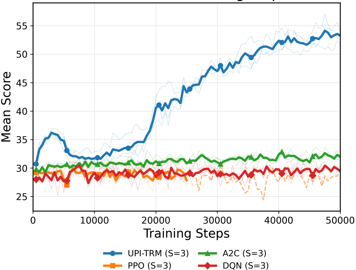
9×9 Sudoku (50k steps) Mean Score vs Training Steps
