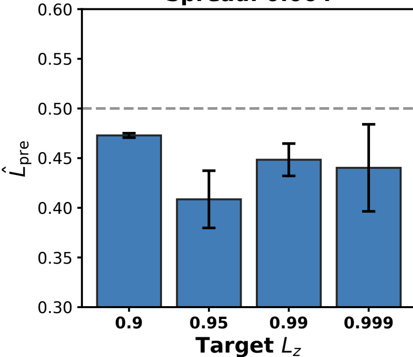
(A) Pre-proj Lipschitz ( R=\infty ) Spread: 0.064
