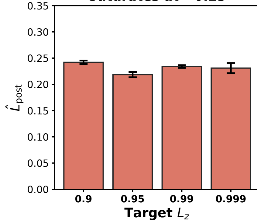
(B) Post-proj Lipschitz ( R=10 ) Saturates at \sim 0.23
