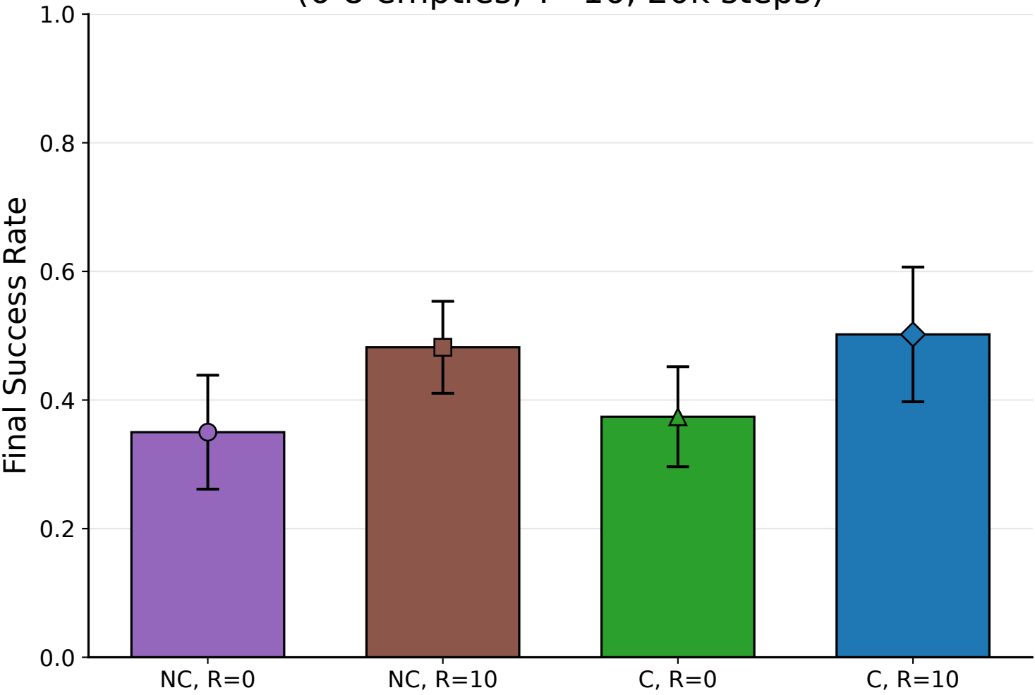
Controlled No-Mask Hard 4x4: Final Success Rates (6-8 empties, T=16, 20k steps)
