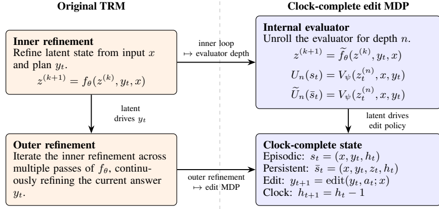
Figure 2: Internal computation and external decisions. TRM refines a latent and then its answer representation (Jolicoeur-Martineau, 2025). UPI-TRM uses the inner recurrence to evaluate a plan and replaces the outer answer update with a checker-rewarded edit. The n recurrent steps occur within one state assessment; each edit advances the environment clock. Carrying the latent between edits changes the Markov state from (x, y, h) to (x, y, z, h) .
