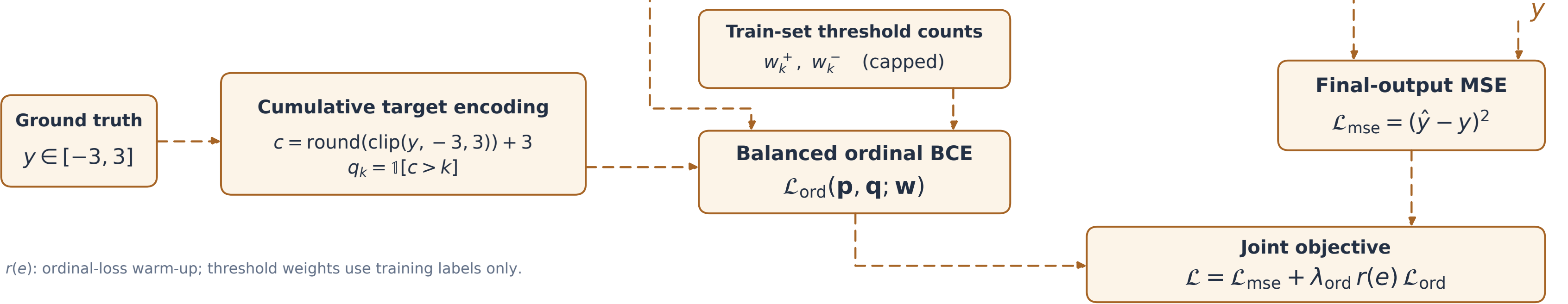
(b) Balanced ordinal supervision and joint optimization
