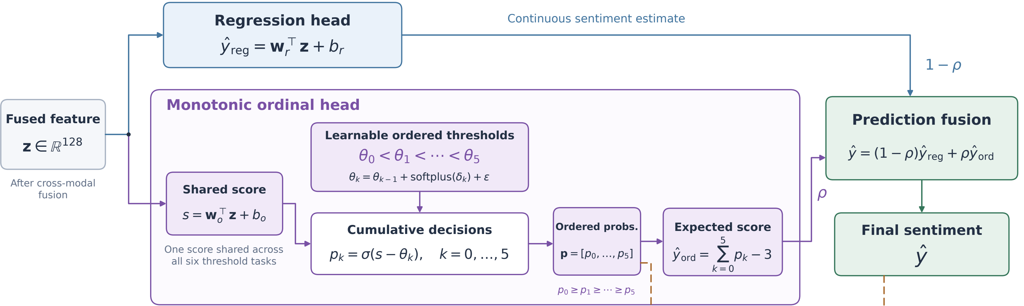
(a) Joint prediction
